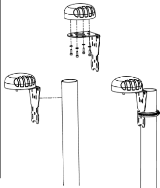
External Pole Mount
