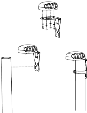
Internal Pole Mount
