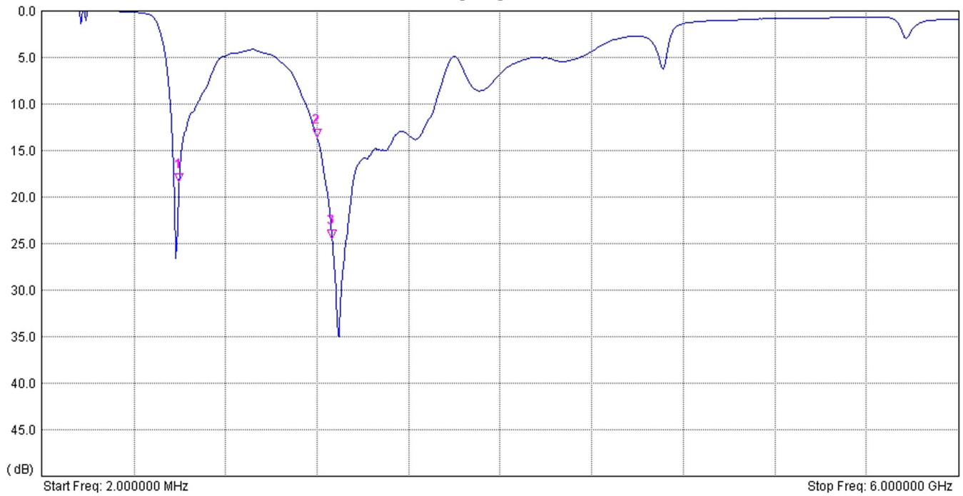
S11 Log Magnitude
